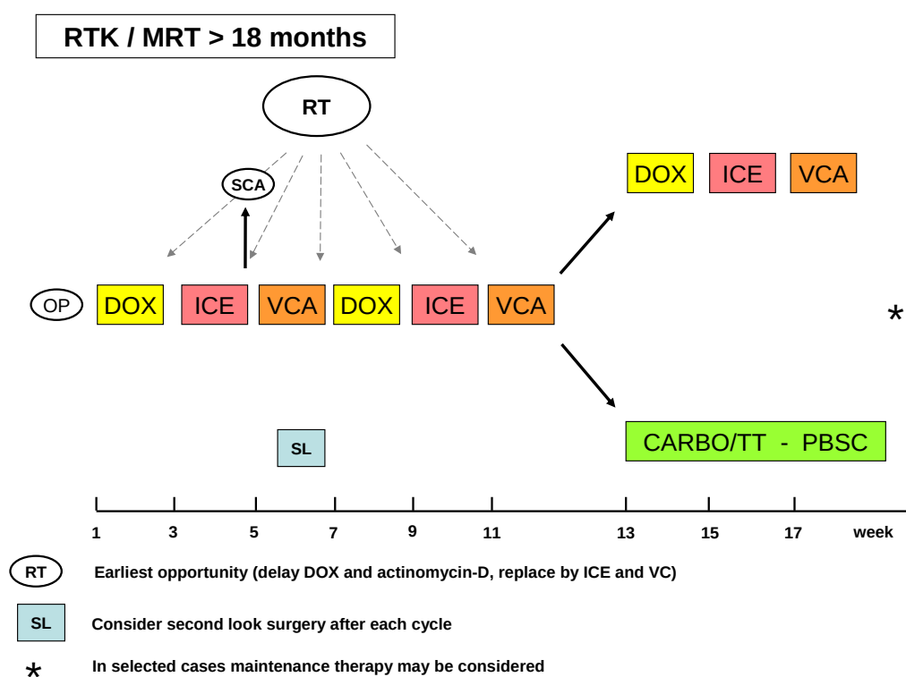
Figure II.6: RTK > 18 months
