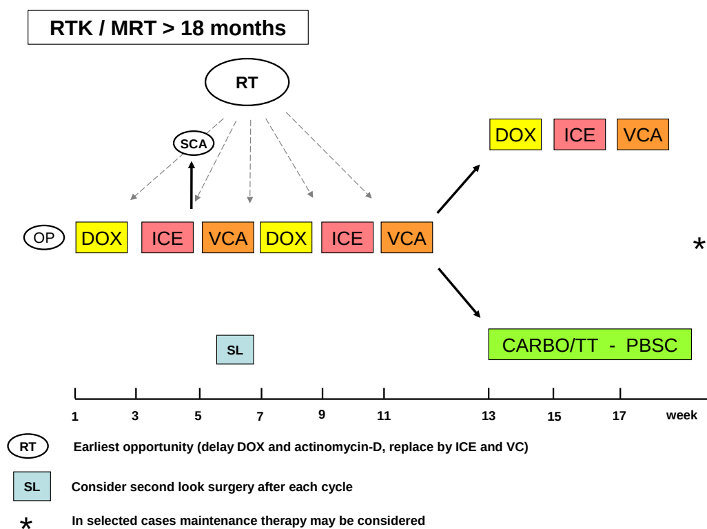
Figure III.6: MRT > 18 months
