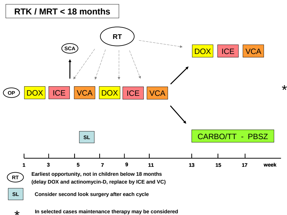
Figure II.5: RTK < 18 months
